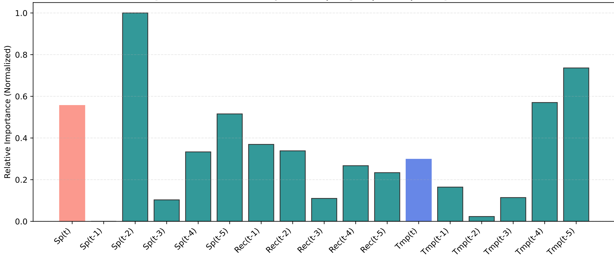
Input Channel Priority: REAL | Lag 5 | MSE | w/ Spawner(t)
