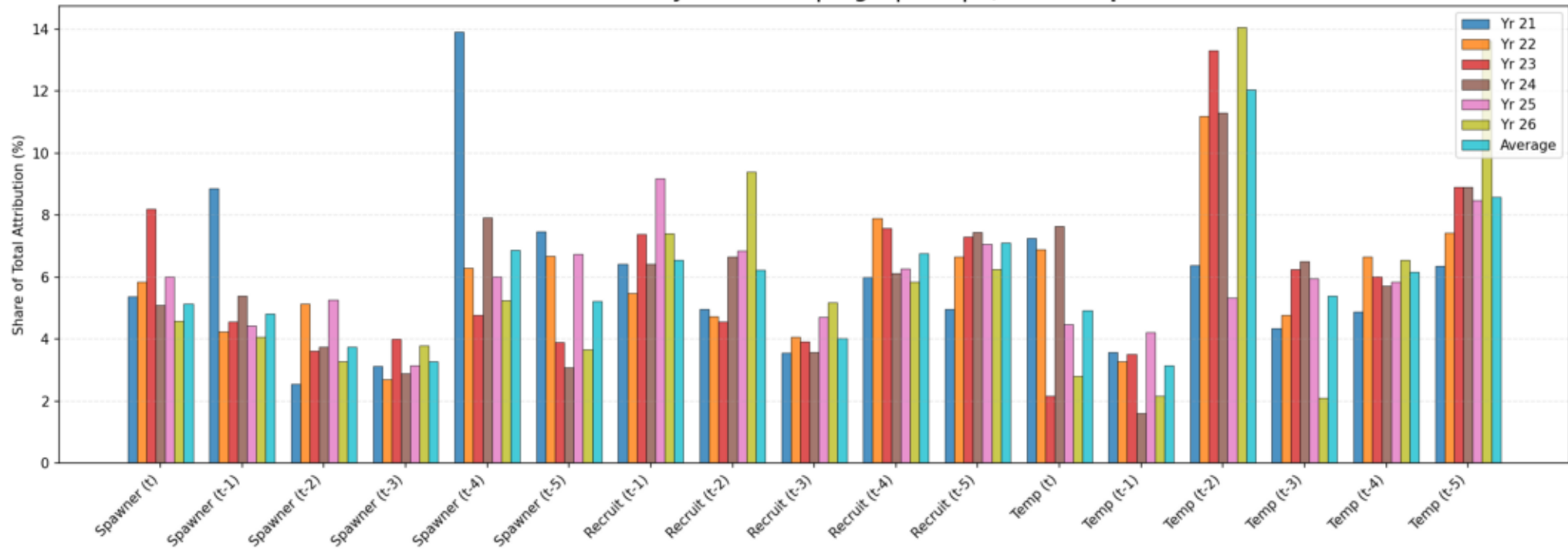
Channel Attribution by Year: REAL | Lag 5 | MSE | w/ Current Spawner
